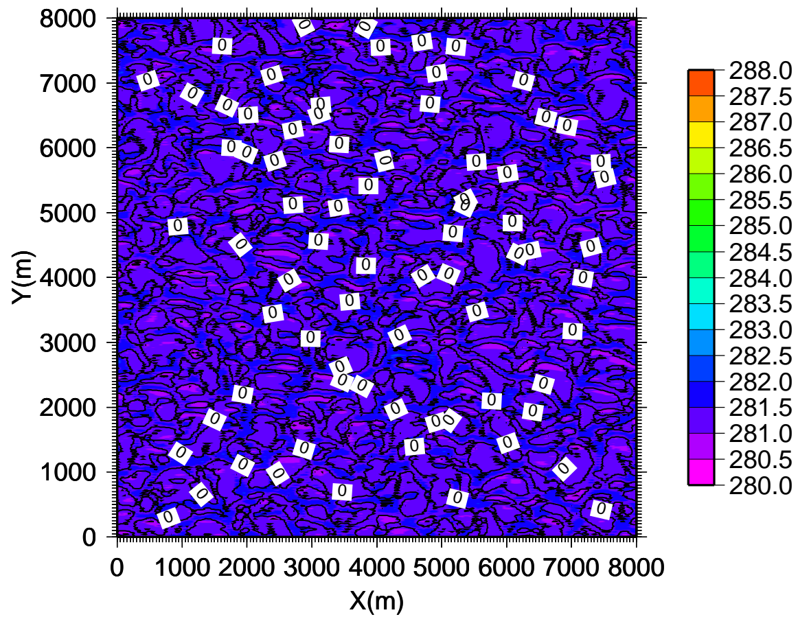
Pt,W(Z=0)
